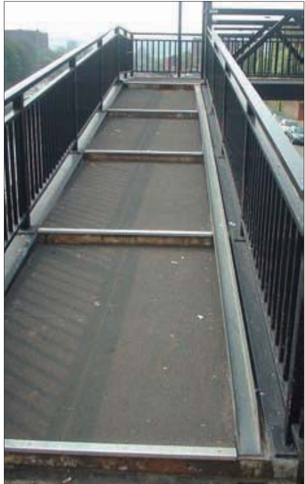
Figure 10.11 Channel section wheeling ramp fitted to existing footbridge (Adrian Lord)
