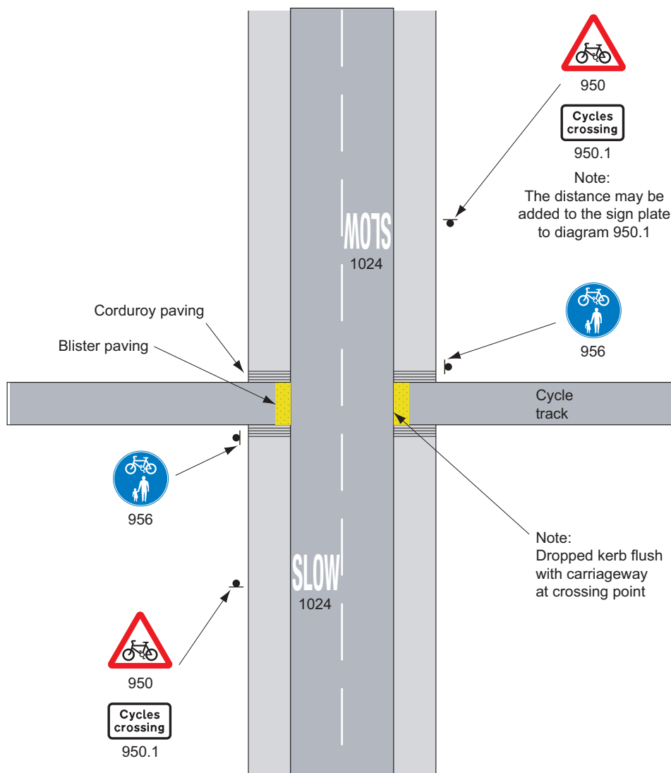
Figure 10.1 Typical cycle crossing
