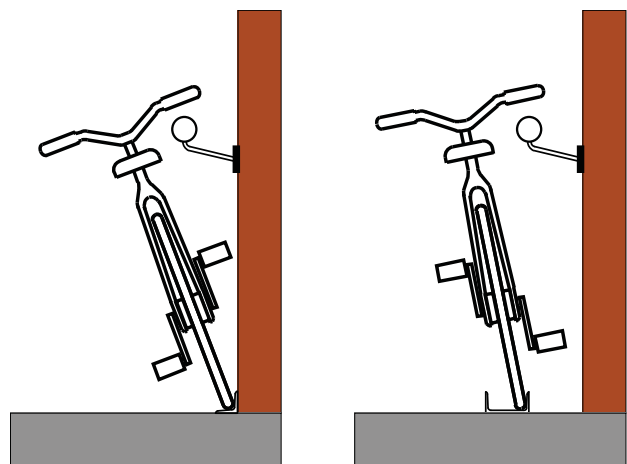
Figure 10.12 Typical wheeling ramp installations
